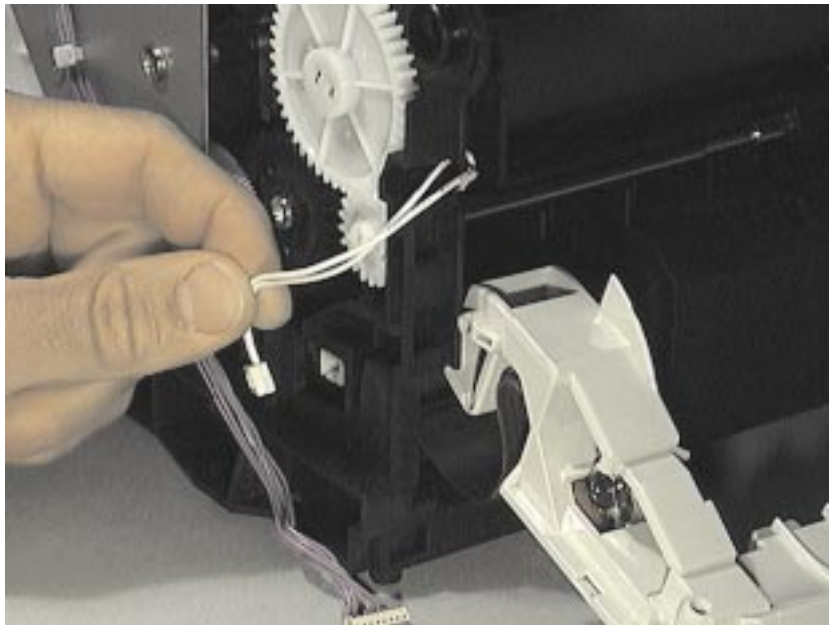
Figure 5-3 Thermistor Connector
