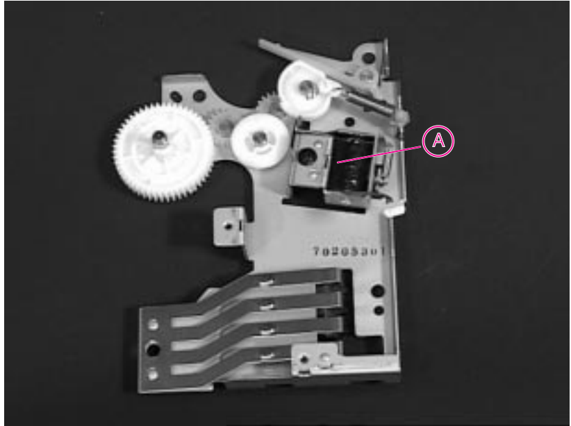
Figure 6-30 Pickup Gear Assembly with Solenoid
