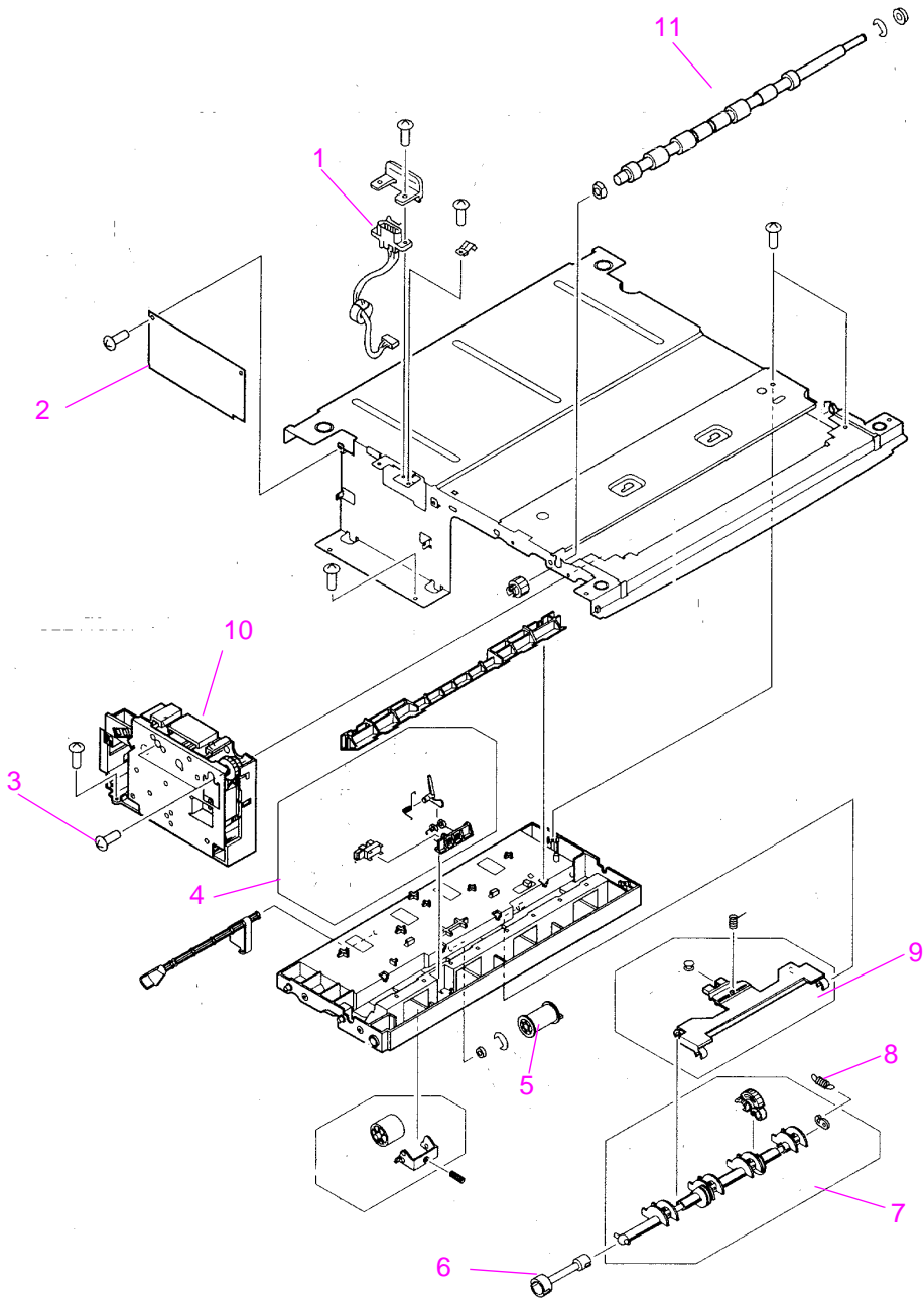
Figure 8-20 500-sheet Feeder (2 of 2)
