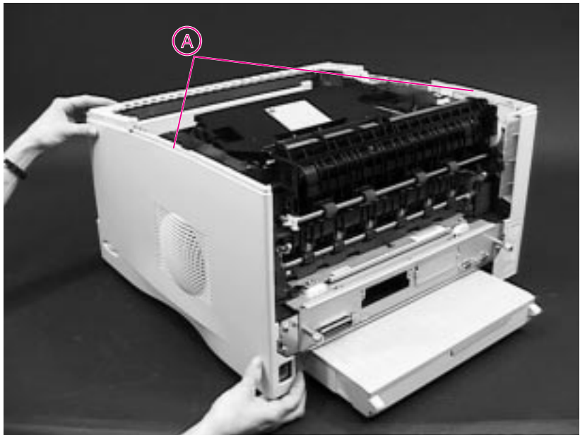
Figure 6-16 Side Covers
