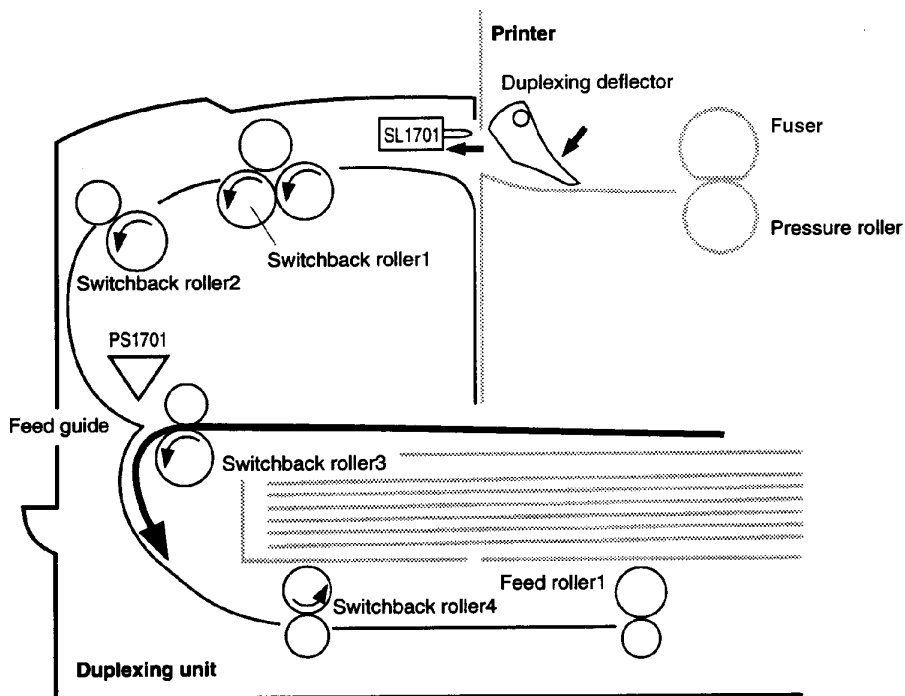
Figure 5-24 Duplexing Unit
