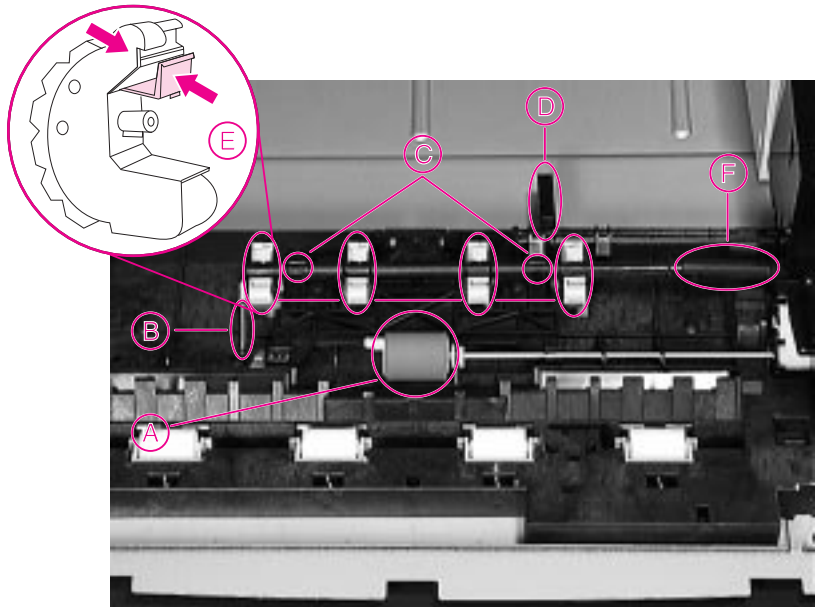
Figure 6-68 Removing the Feed Roller and D-rollers
