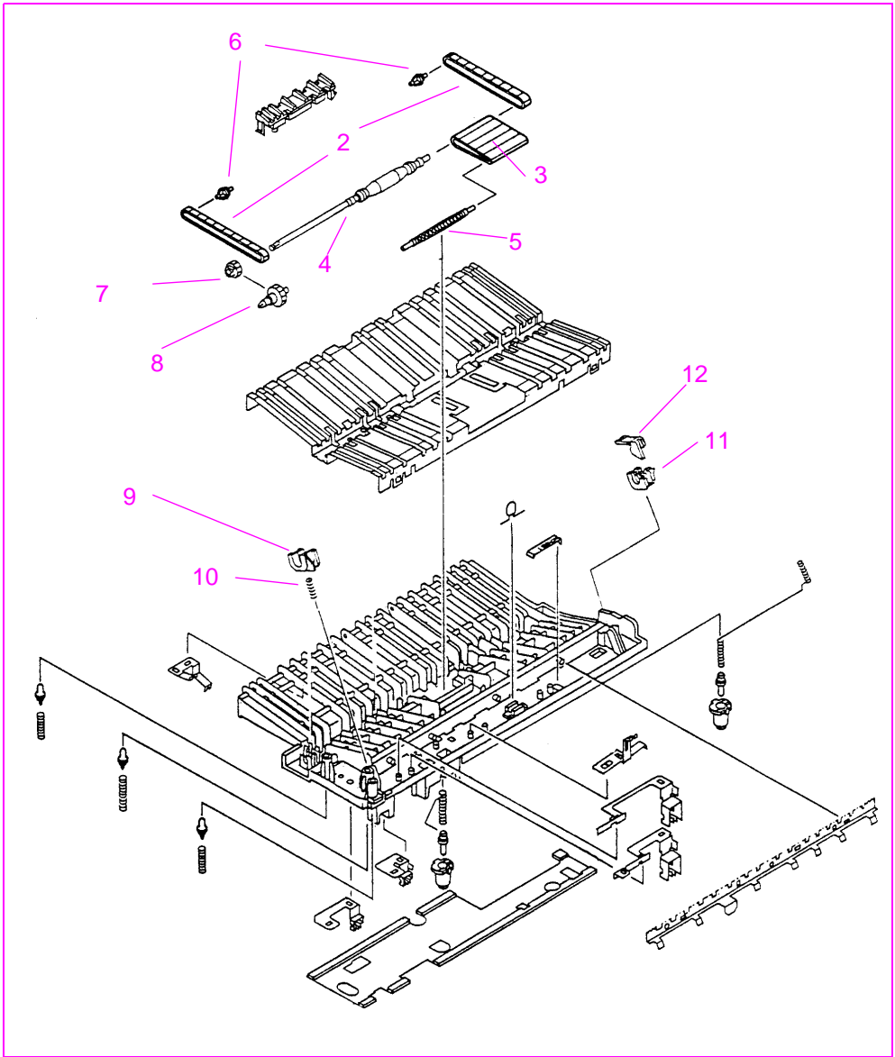
Figure 8-10 Paper Feed Belt Assembly
