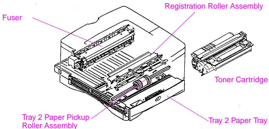
Figure 8-1 Assembly Locations
