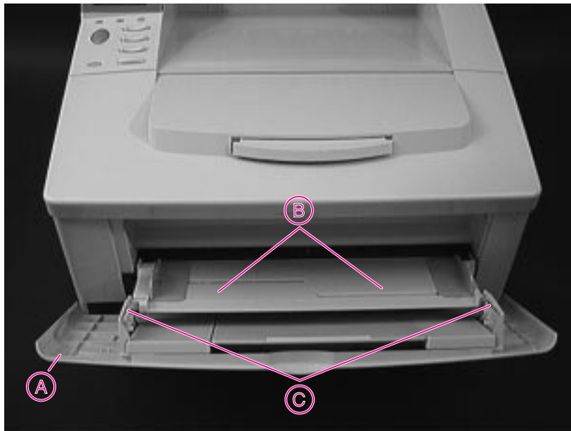
Figure 6-11 Front Cover
