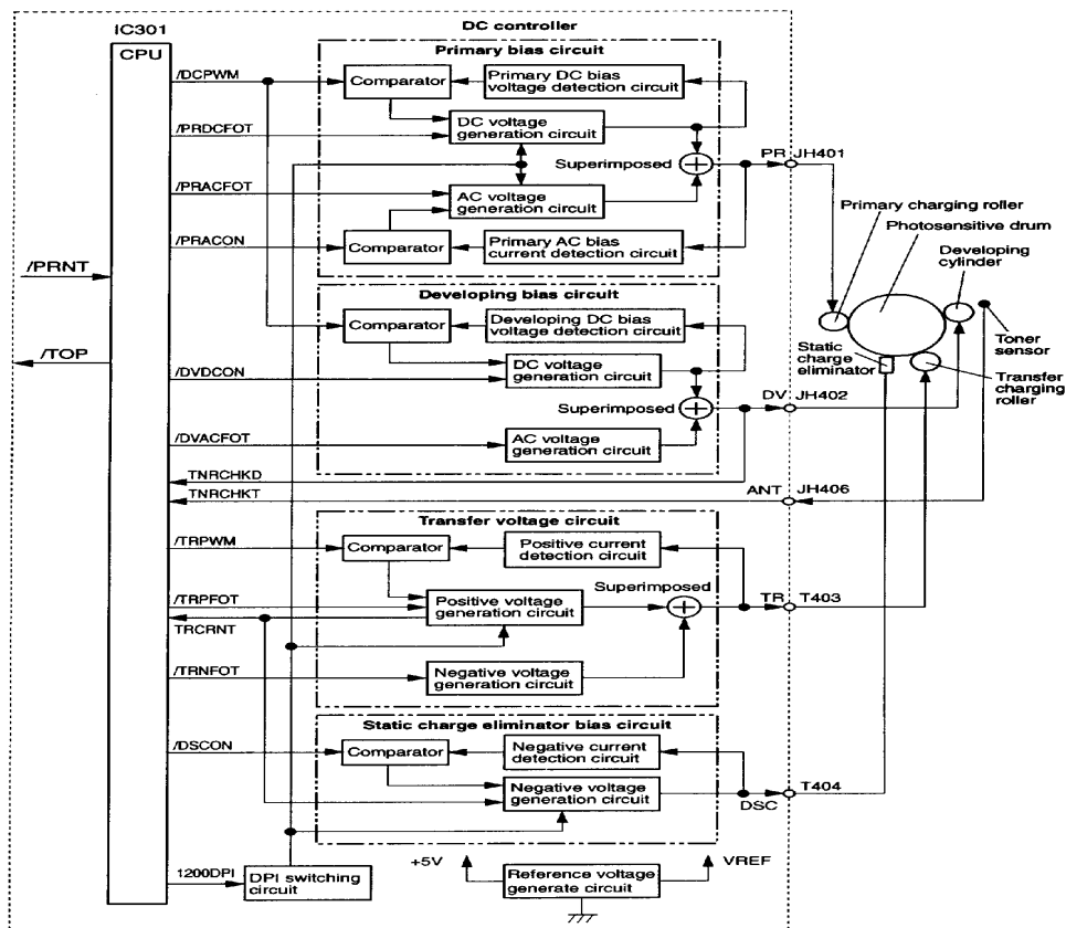
Figure 5-3 High-voltage Power Supply Circuit
