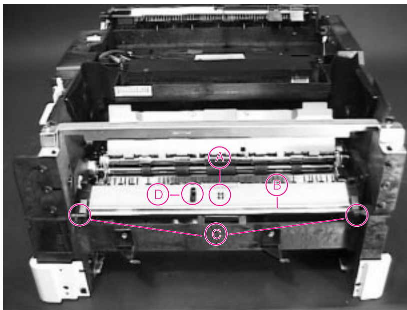
Figure 6-46 Tray 1 Lift Plate
