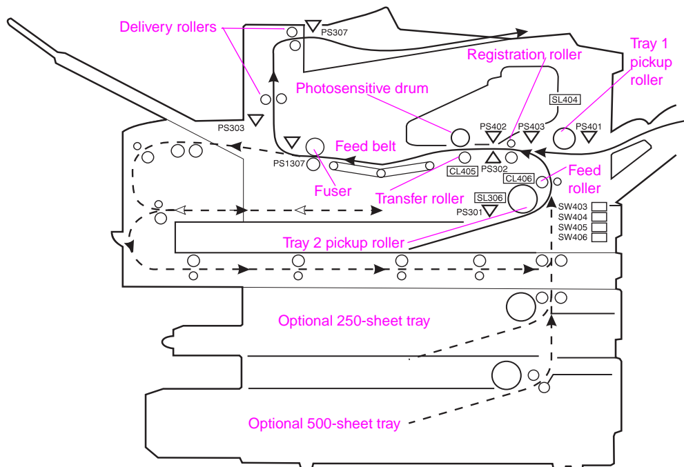
Figure 7-17 Paper Path and Components
