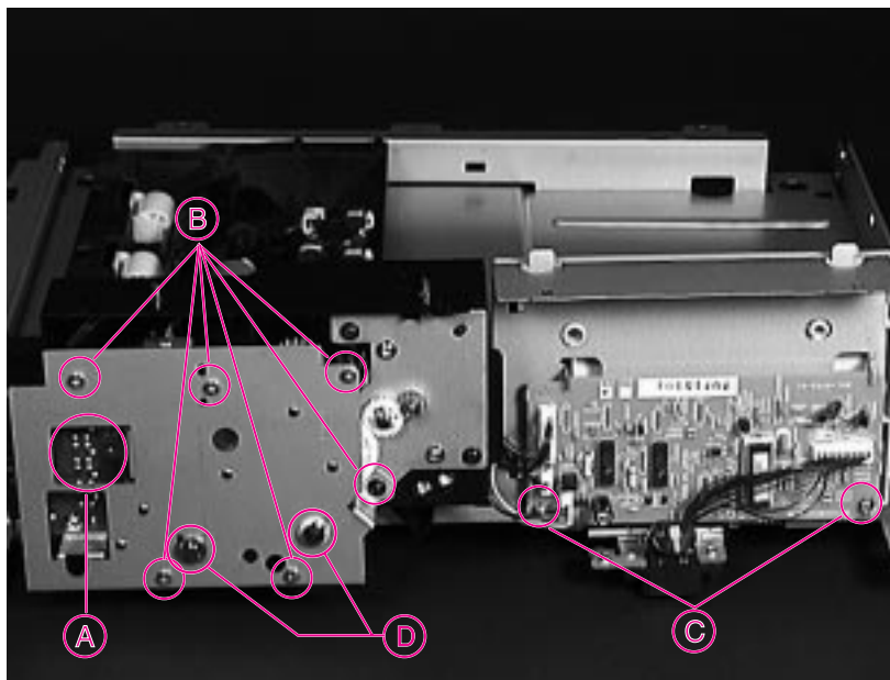
Figure 6-69 Removing the Gear Assembly and PCA
