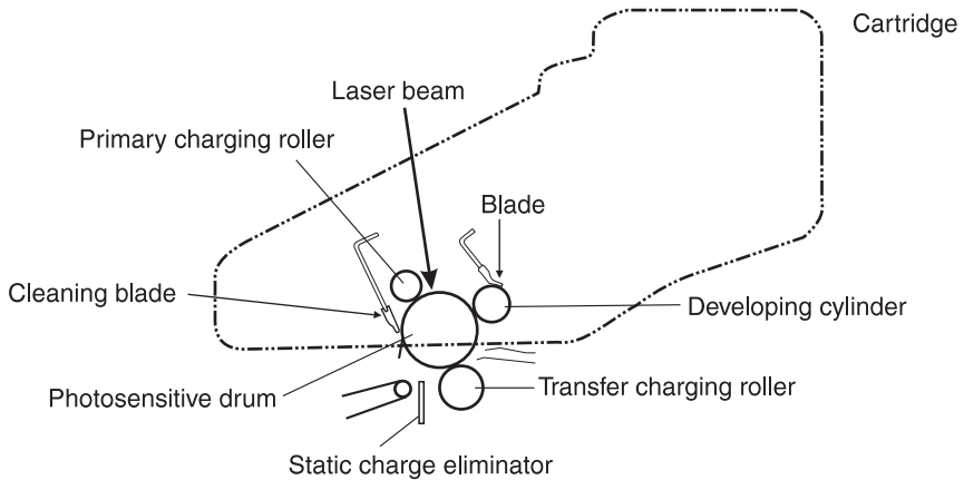
Figure 5-7 Toner Cartridge
