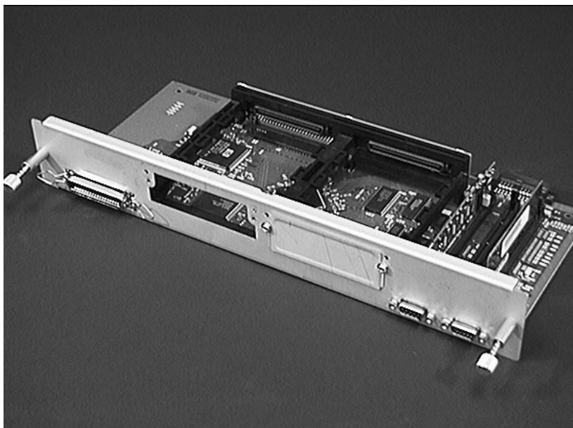
Figure 6-32 Formatter Assembly
