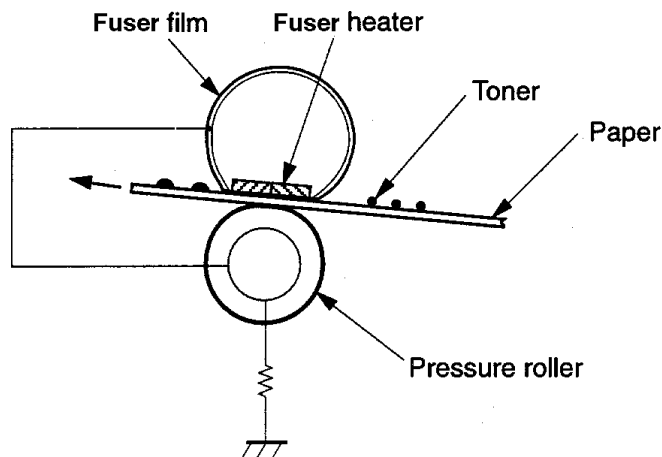
Figure 5-14 Image Fusing
