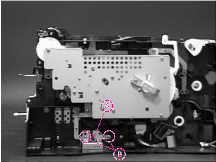
Figure 6-52 Power Connection
