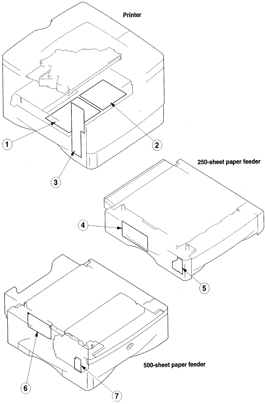
Figure 7-25 PCA's
