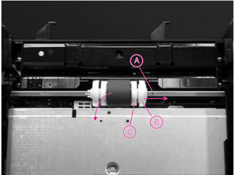
Figure 6-34 Tray 2 Roller (bottom view of printer)
