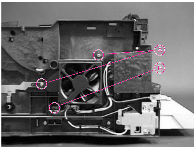
Figure 6-31 Fan (right side view of printer)
