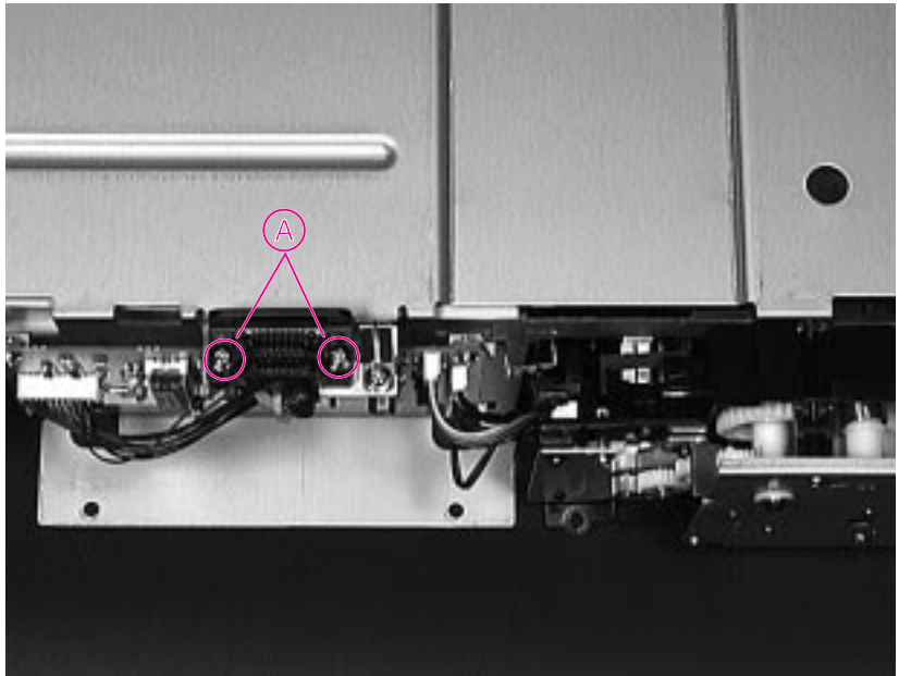
Figure 6-70 Removing the Power Connector
