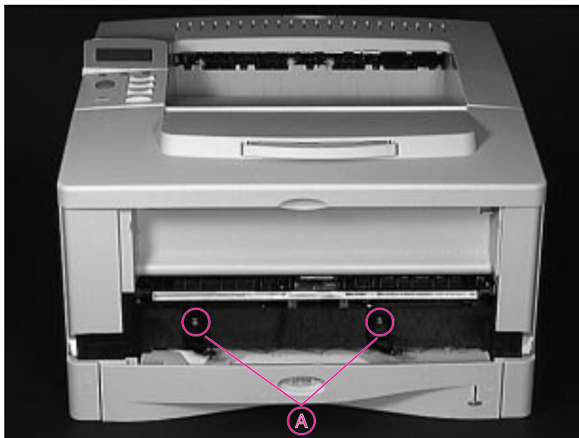
Figure 6-13 Front Cover Pins
