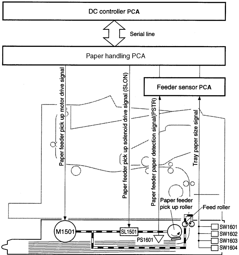
Figure 7-11 Tray 2 Paper Path
