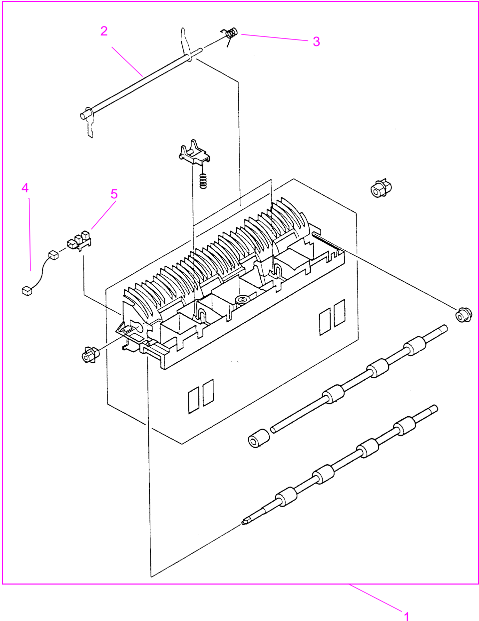
Figure 8-11 Paper Feed Roller Assembly
