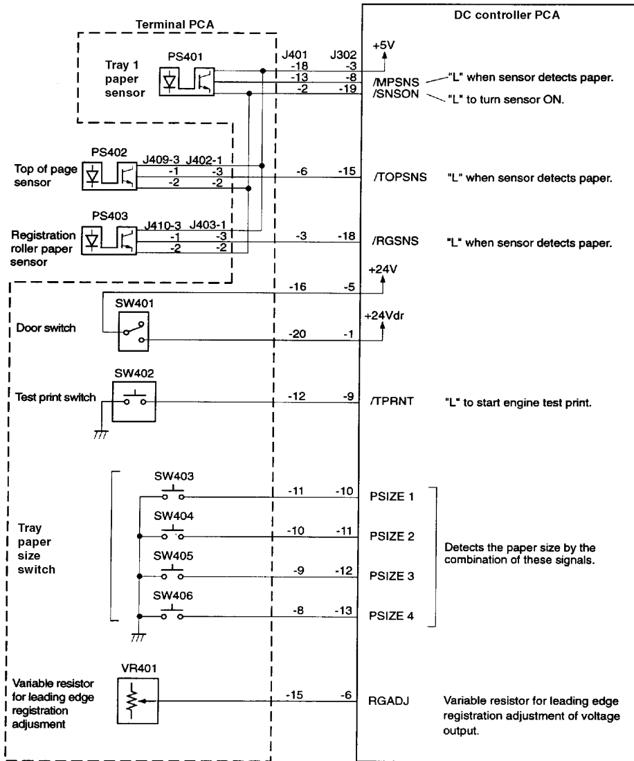
Figure 7-33 DC Controller PCA I/O (1 of 4)
