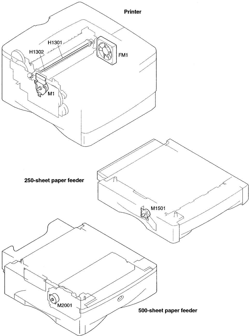
Figure 7-21 Motors
