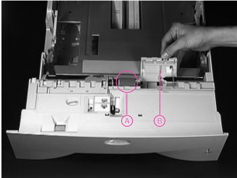
Figure 6-71 Removing the Separation Roller
