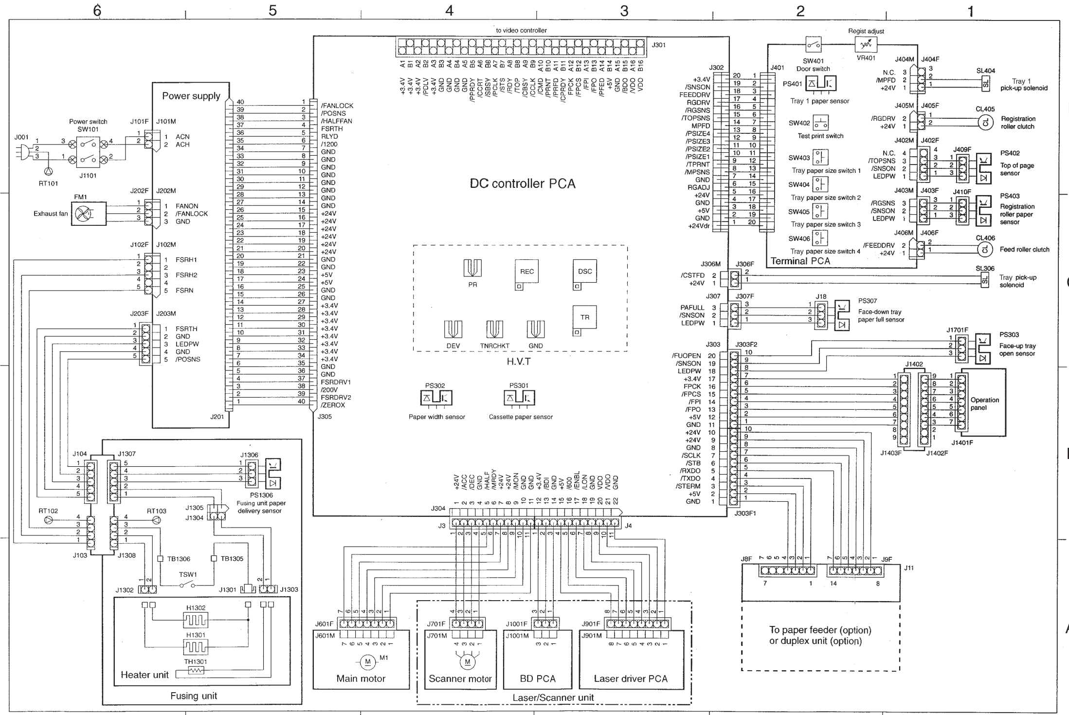
Wiring Diagram HP LaserJet 5000, 5000 N, 5000 GN, and 5000 LE Printers
