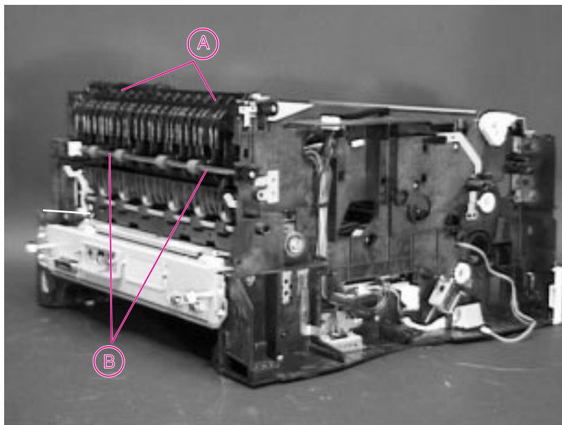
Figure 6-55 Upper Delivery Assembly (rear left view of printer)
