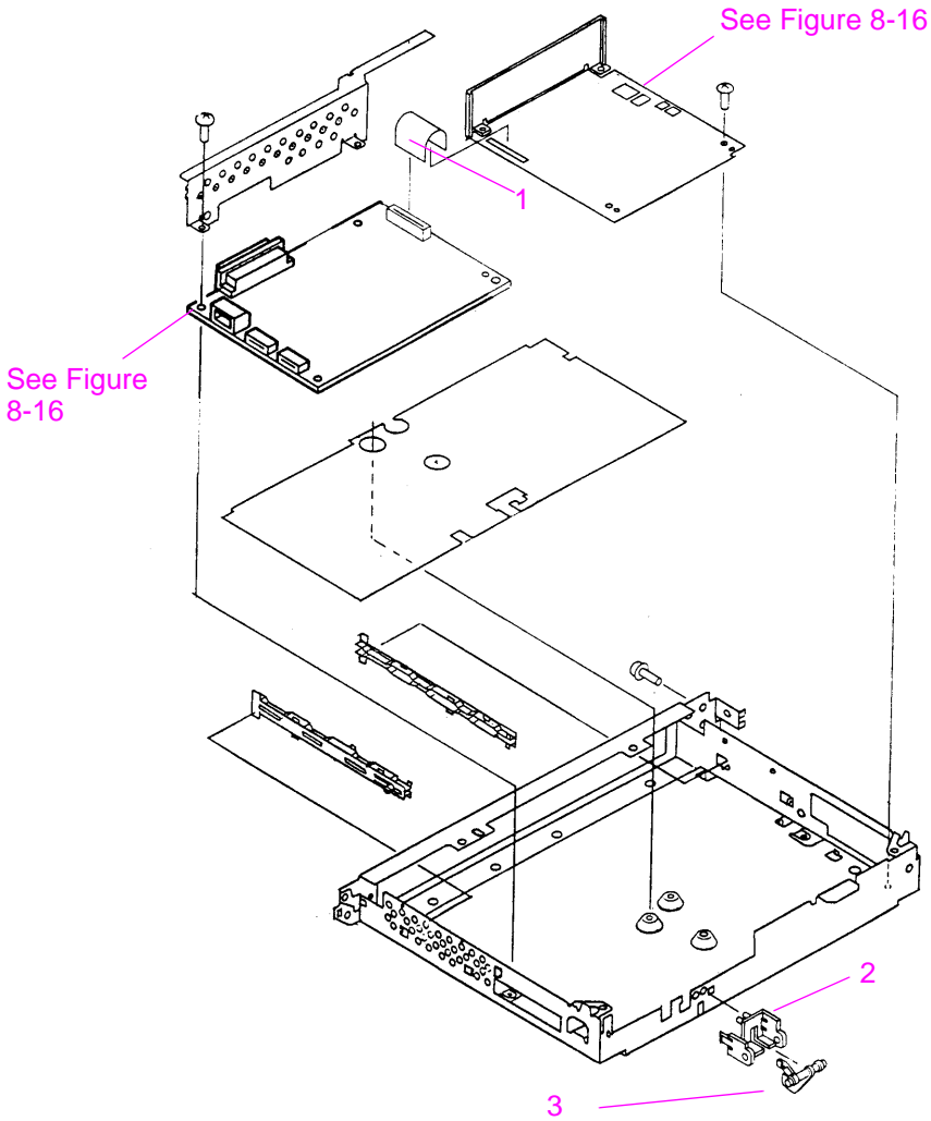
Figure 8-17 Printer Controller Assembly
