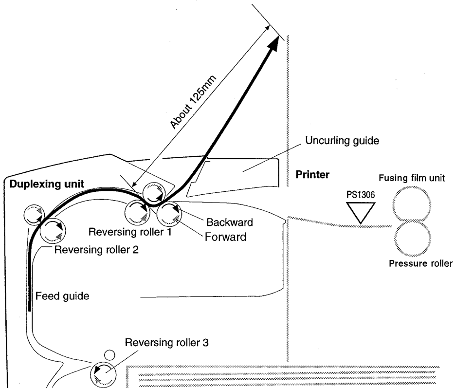
Figure 5-26 Dance Mode
