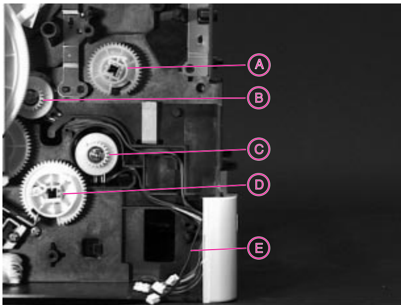
Figure 6-35 Paper Feed Roller Clutch (left side view of printer)
