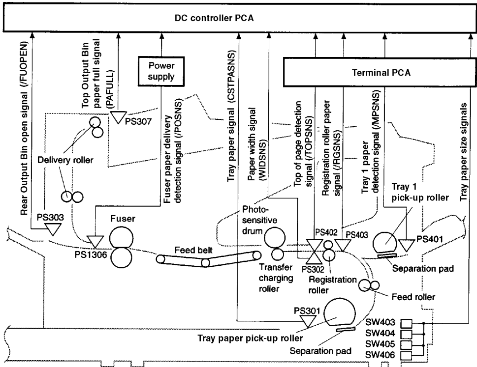
Figure 5-16 Paper Path
