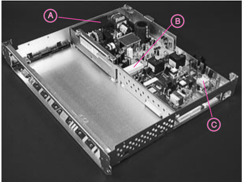
Figure 6-40 DC Controller Assembly
