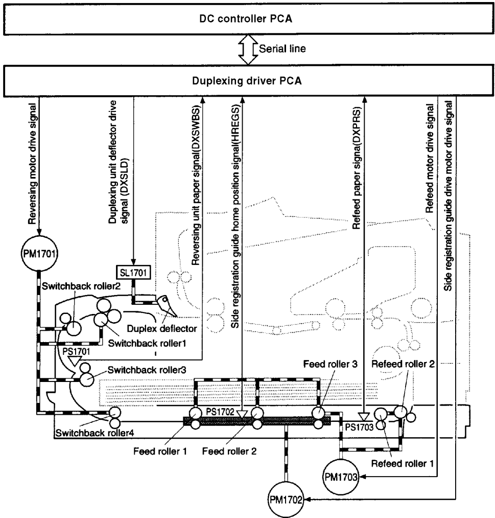
Figure 7-16 Duplexing Unit
