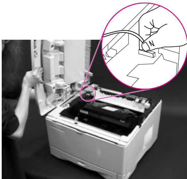
Figure 6-7 Control Panel Cable
