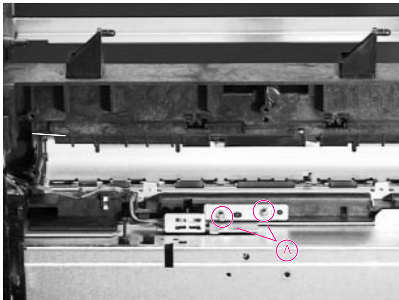
Figure 6-49 Paper Path Detect Sensor
