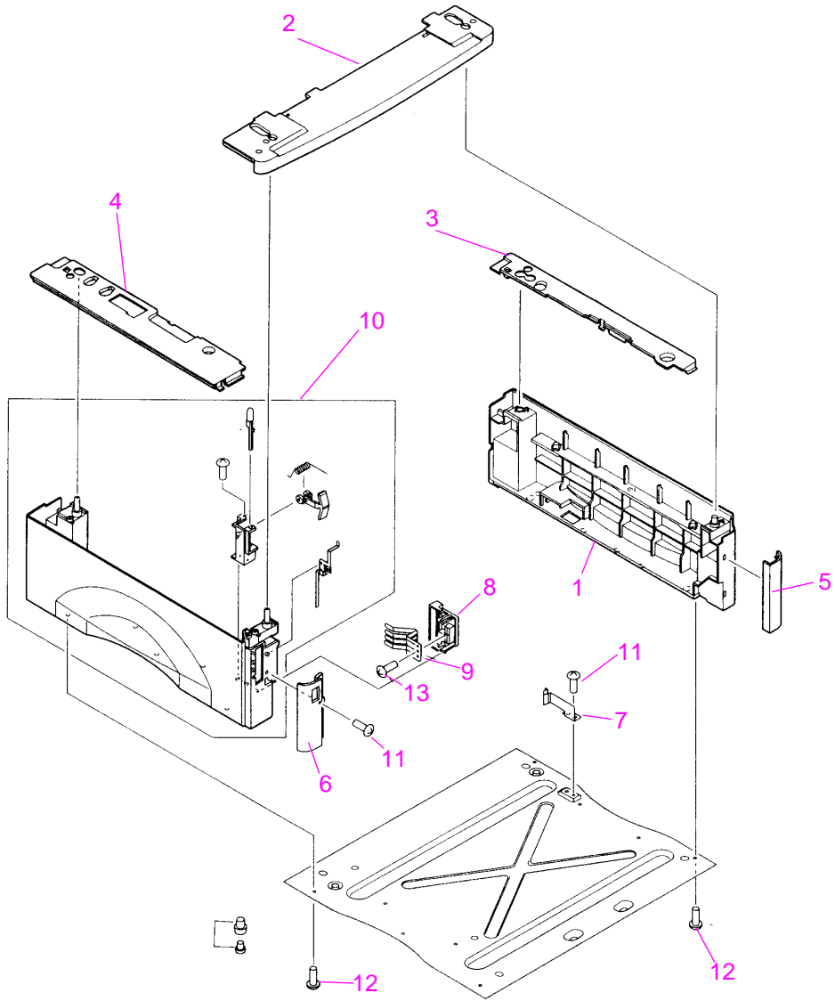
Figure 8-19 500-sheet Feeder (1 of 2)
