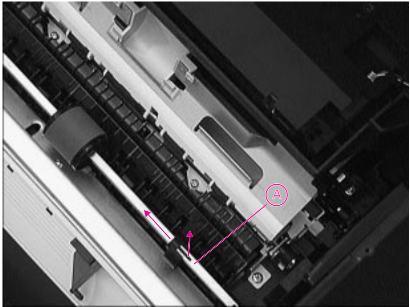
Figure 6-43 Tray 1 Shaft (right side view of printer)
