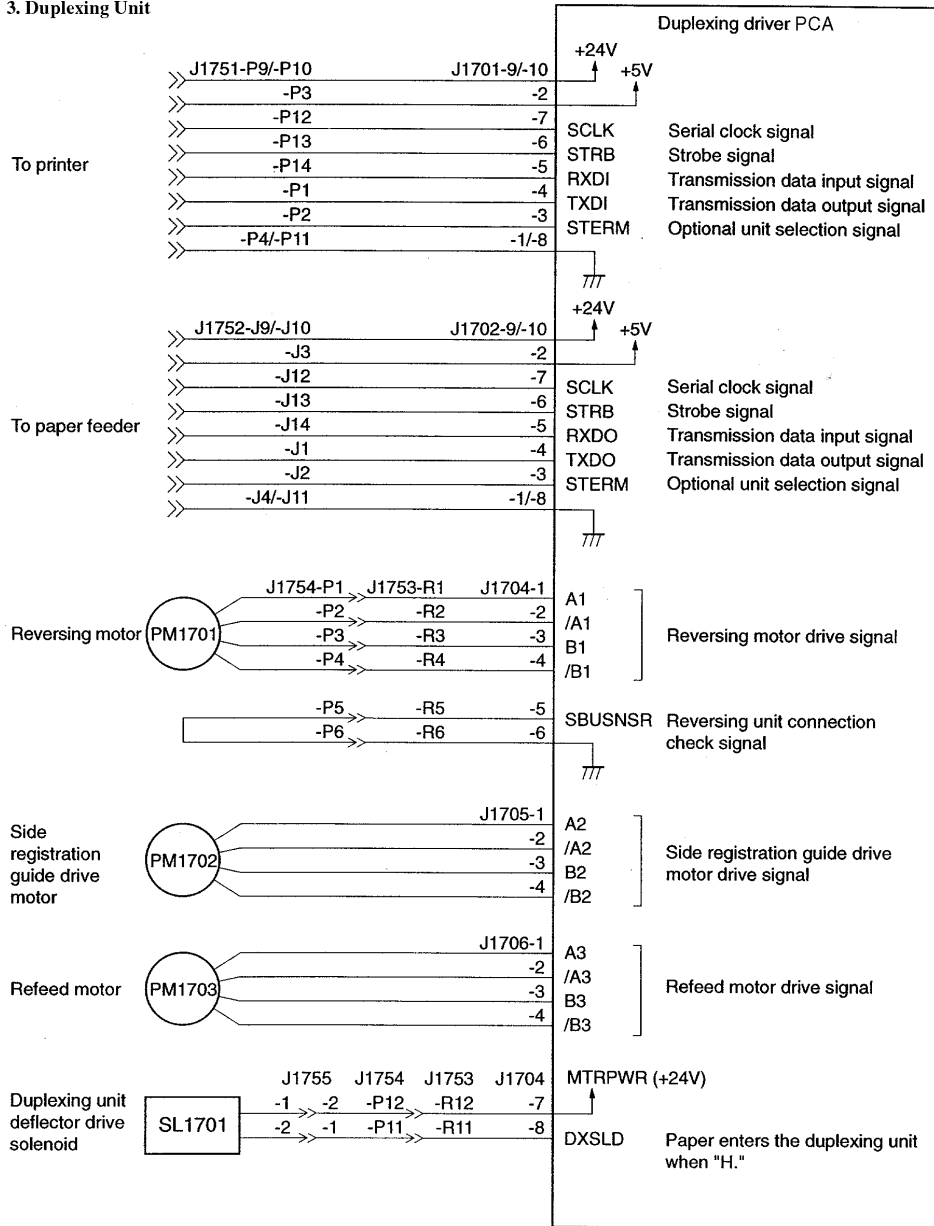
Figure 7-14 Duplexing Unit
