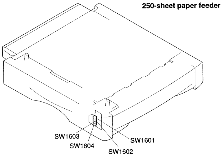
Figure 7-29 Switches
