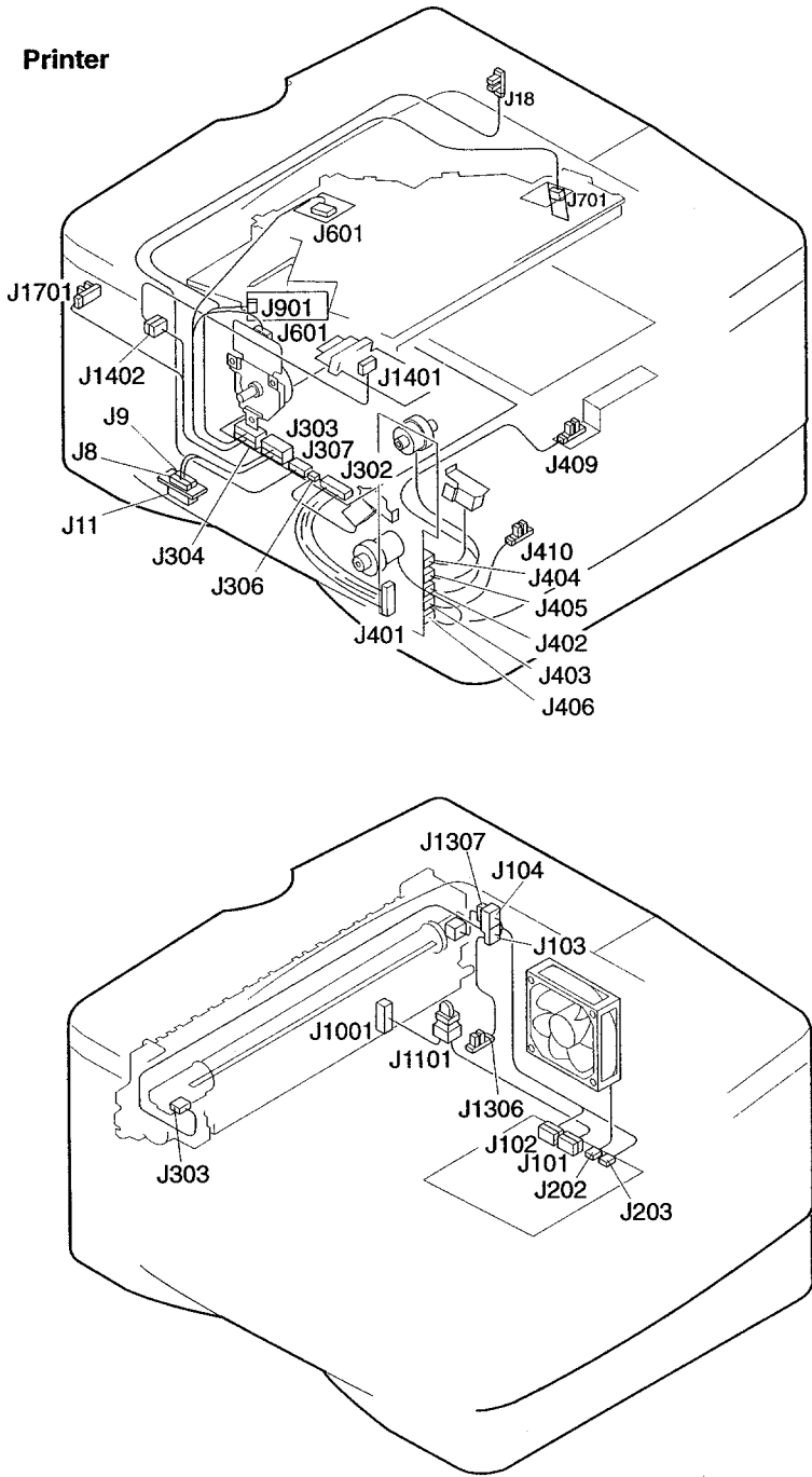
Figure 7-23 Connectors
