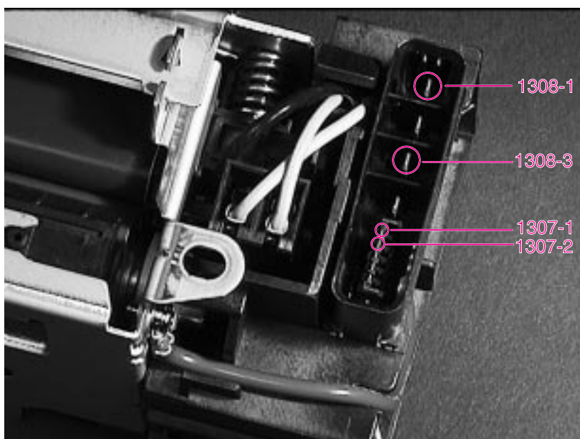
Figure 7-3 Fuser Connectors
