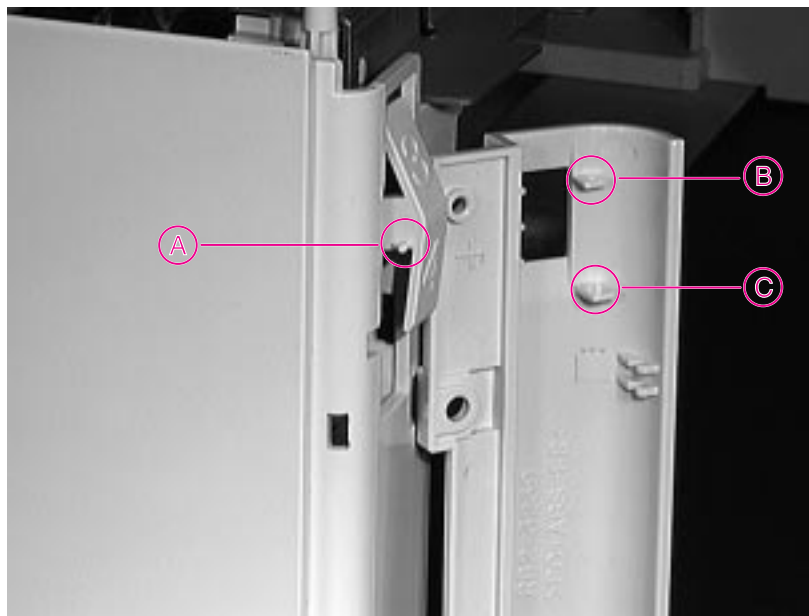
Figure 6-66 Installing the Left Front Corner Cover
