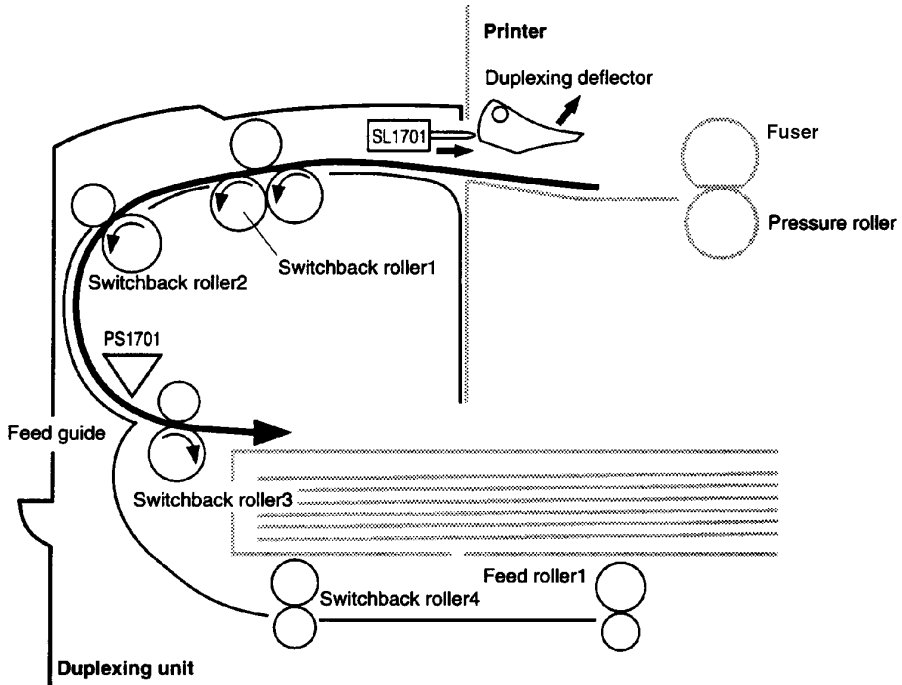
Figure 5-23 Duplexing Unit
