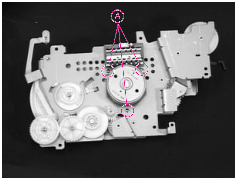
Figure 6-60 Main Gear Assembly with Motor (rear view)
