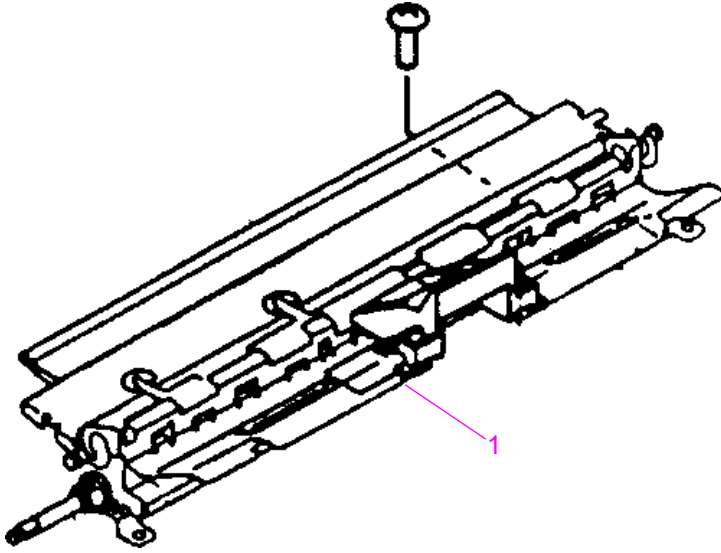
Figure 8-12 Registration Roller Assembly
