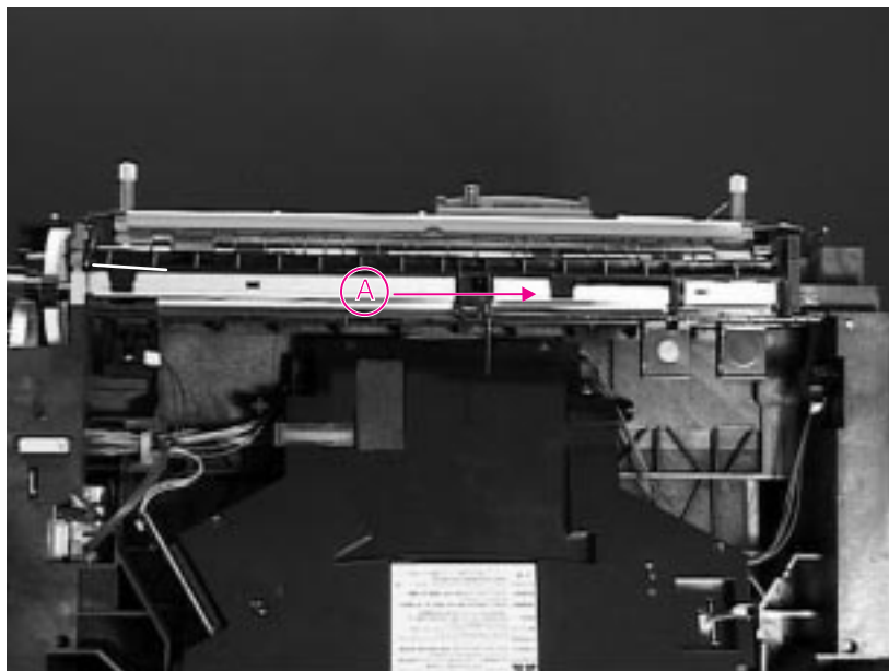
Figure 6-50 Face Down Bin Full Sensor
