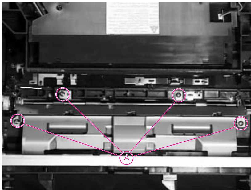
Figure 6-53 Registration Assembly
