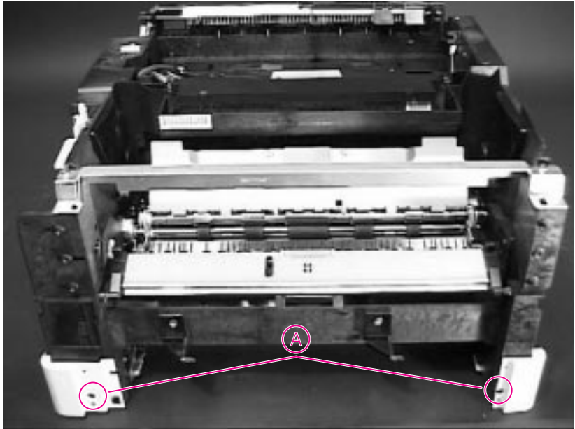
Figure 6-19 Right and Left Corner Covers
