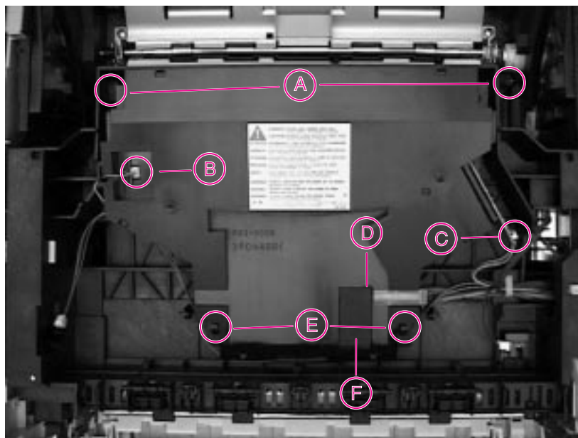
Figure 6-59 Laser Scanner Assembly (top inside view of printer)
