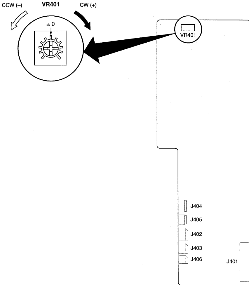
Figure 6-26 Location of VR401
