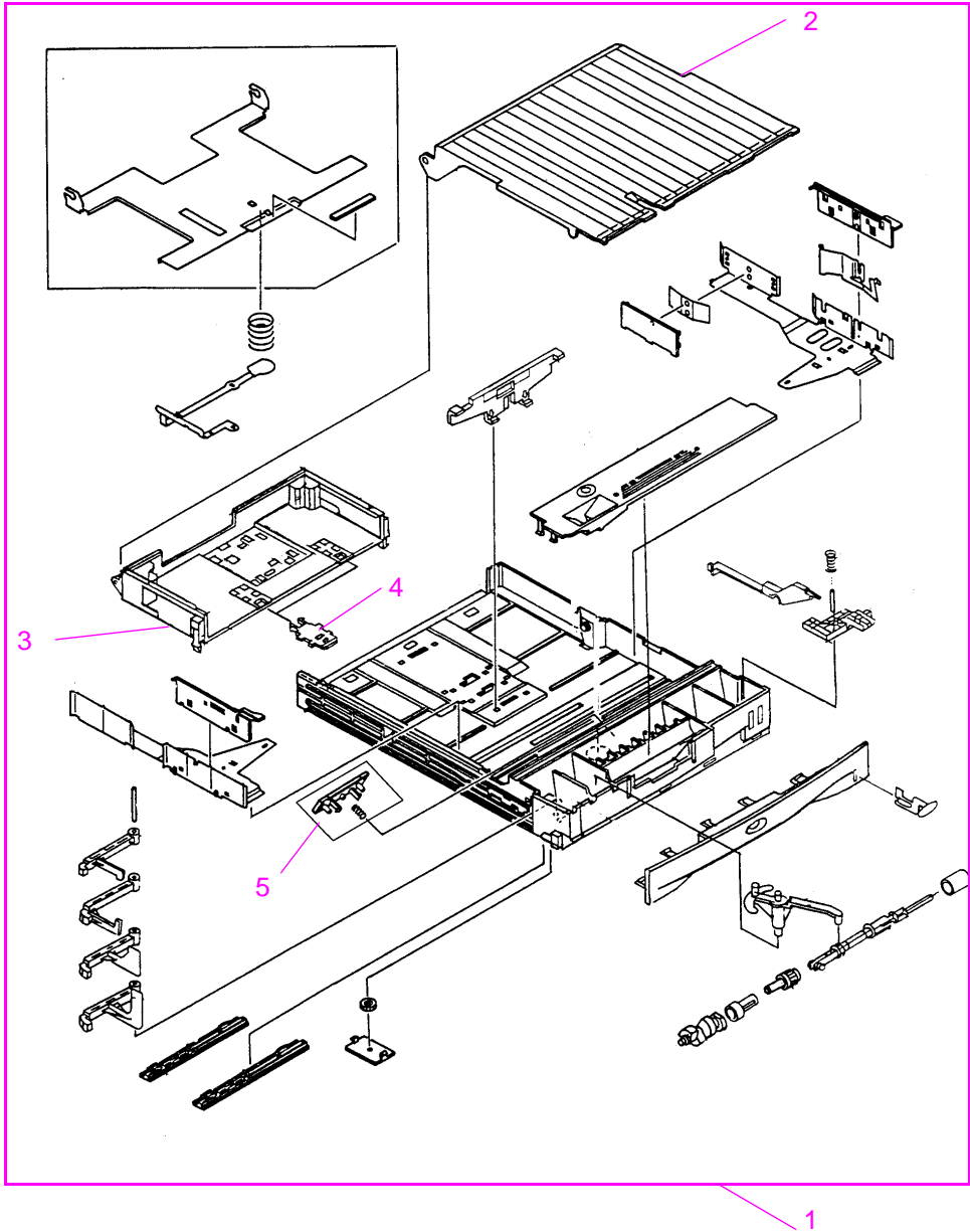
Figure 8-13 250-sheet Universal Tray
