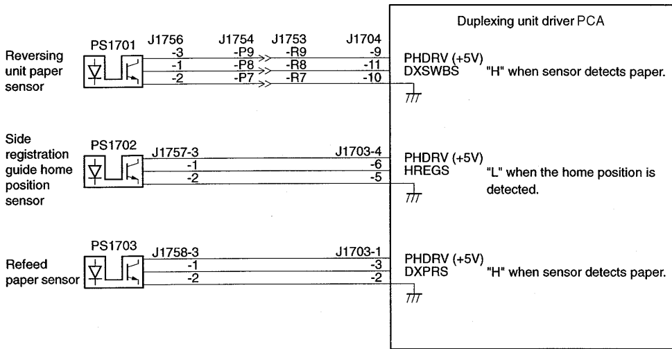
Figure 7-15 Duplexing Unit
