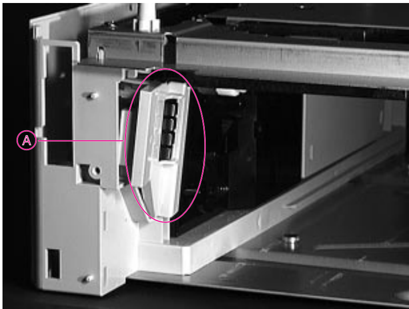
Figure 6-67 Removing the Paper Size Spring Assembly
