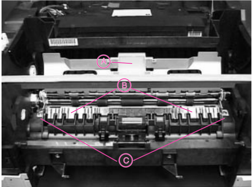
Figure 6-48 Paper Guide
