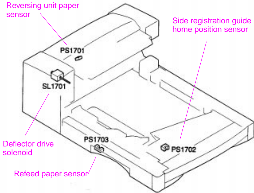
Figure 7-20 Duplexer Sensors and Switches
