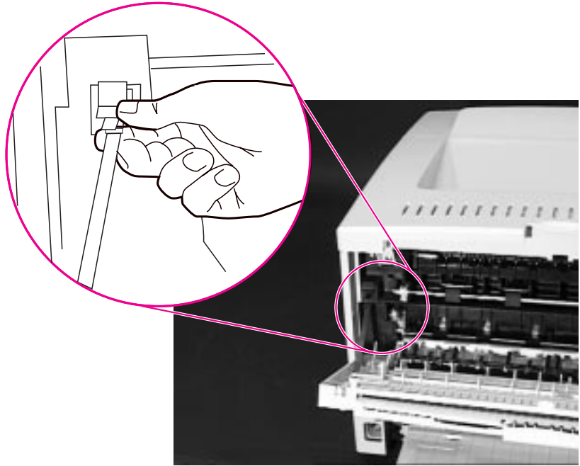
Figure 6-4 Support Strap
