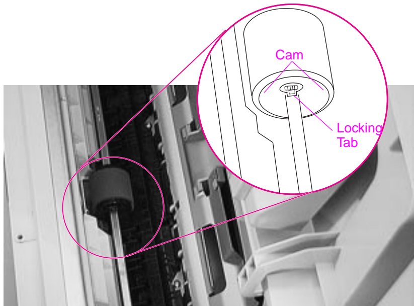
Figure 6-33 Tray 1 Roller
