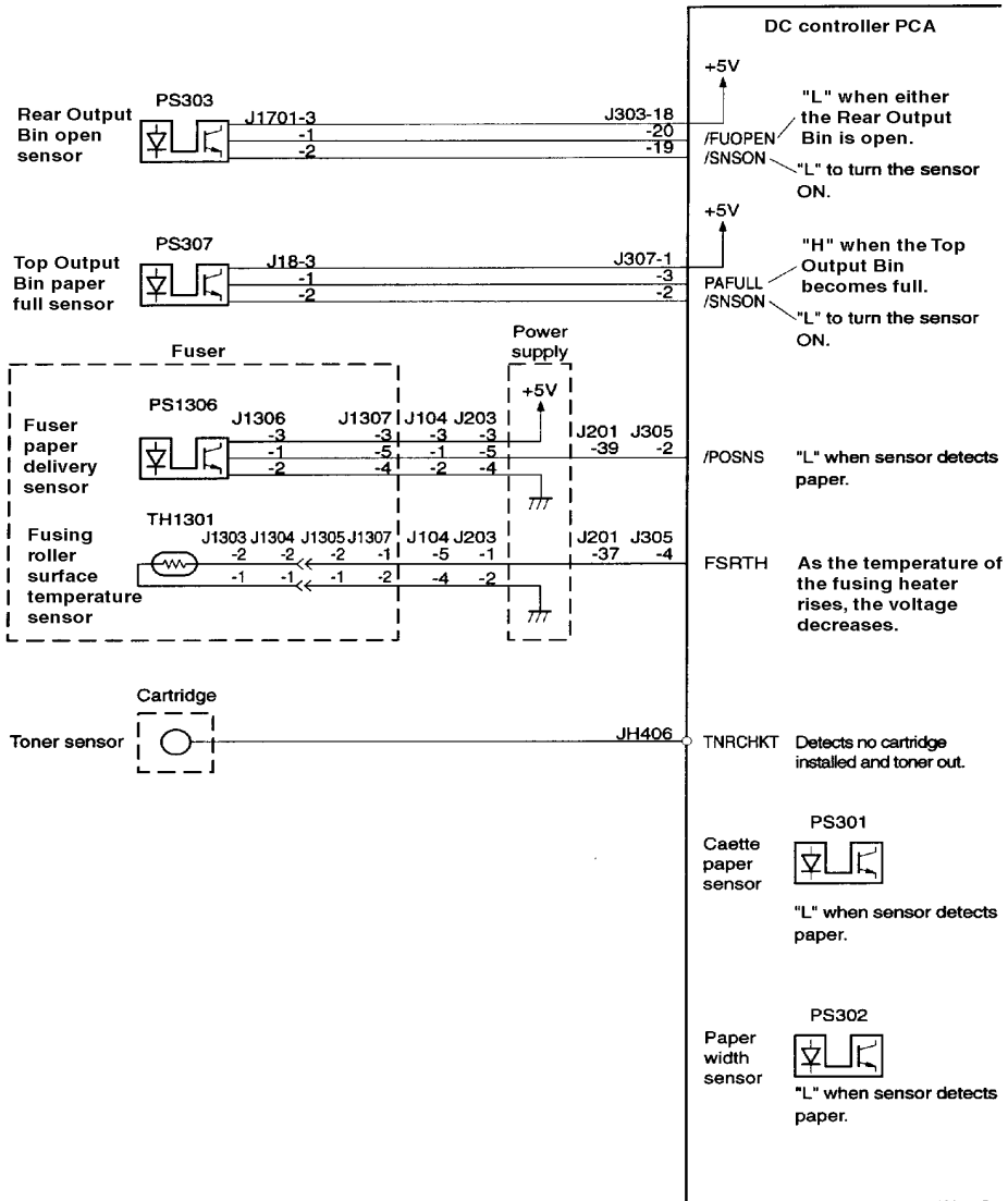
Figure 7-34 DC Controller PCA I/O (2 of 4)
