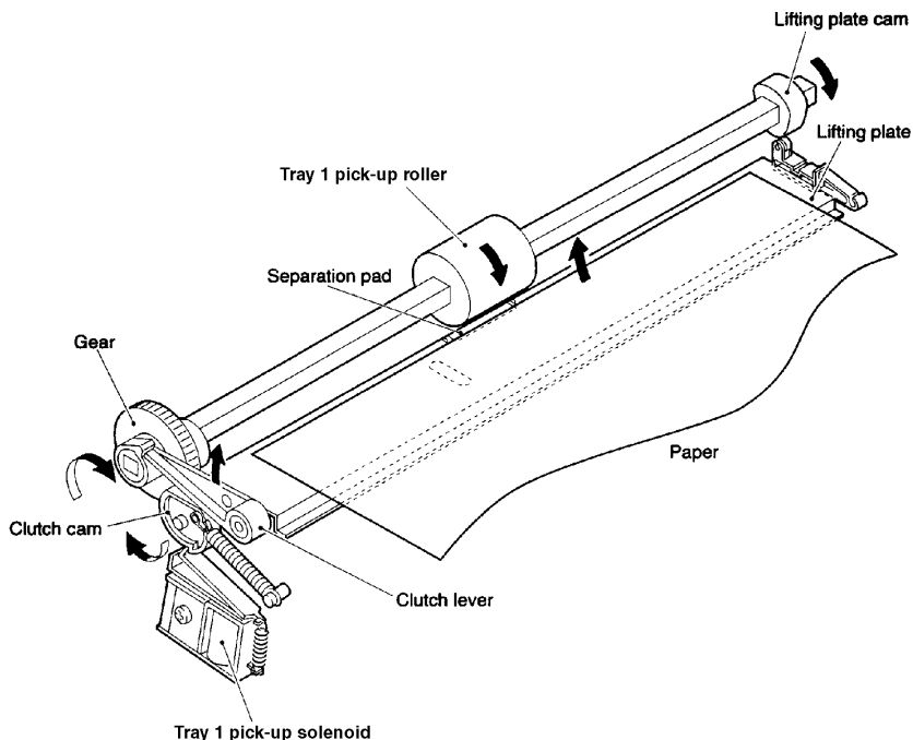
Figure 5-17 Tray 1 Pickup
