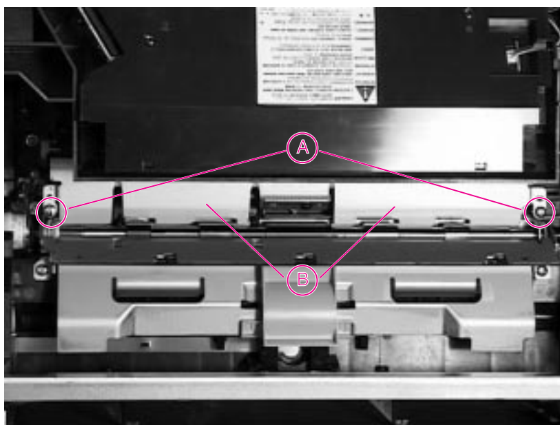
Figure 6-21 Transfer Guide Removal
