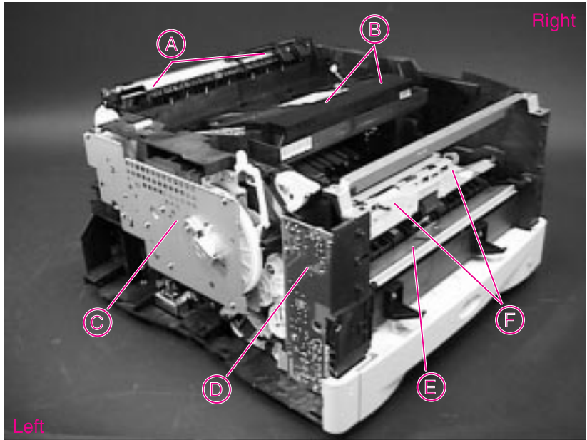
Figure 6-20 Internal Assemblies
