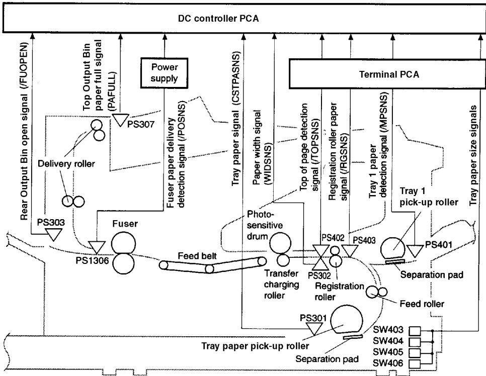
Figure 7-8 Paper Path
