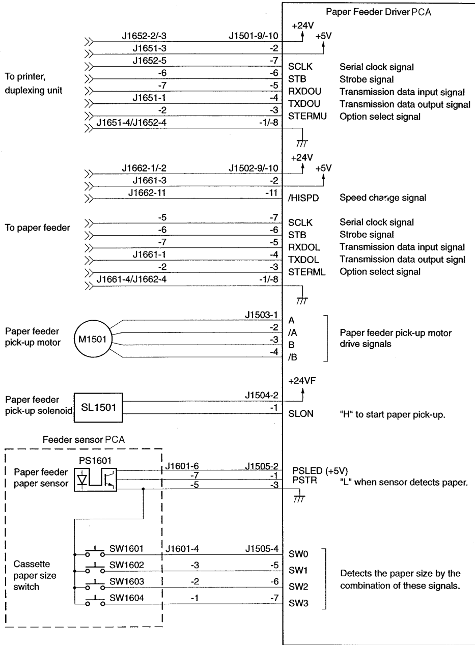
Figure 7-10 250-sheet Paper Feeder
