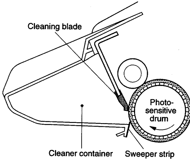
Figure 5-9 Cleaning the Drum
