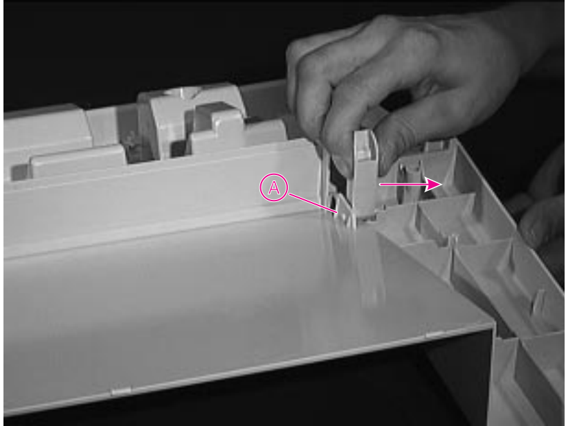
Figure 6-10 Toner Cartridge Door Assembly (Under Side of Top Cover Door)
