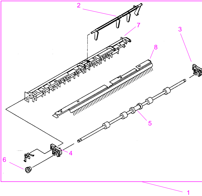
Figure 8-8 Upper Delivery Assembly
