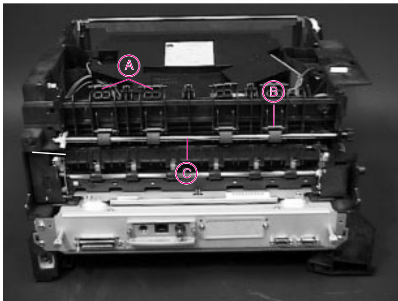
Figure 6-57 Delivery Roller Components
