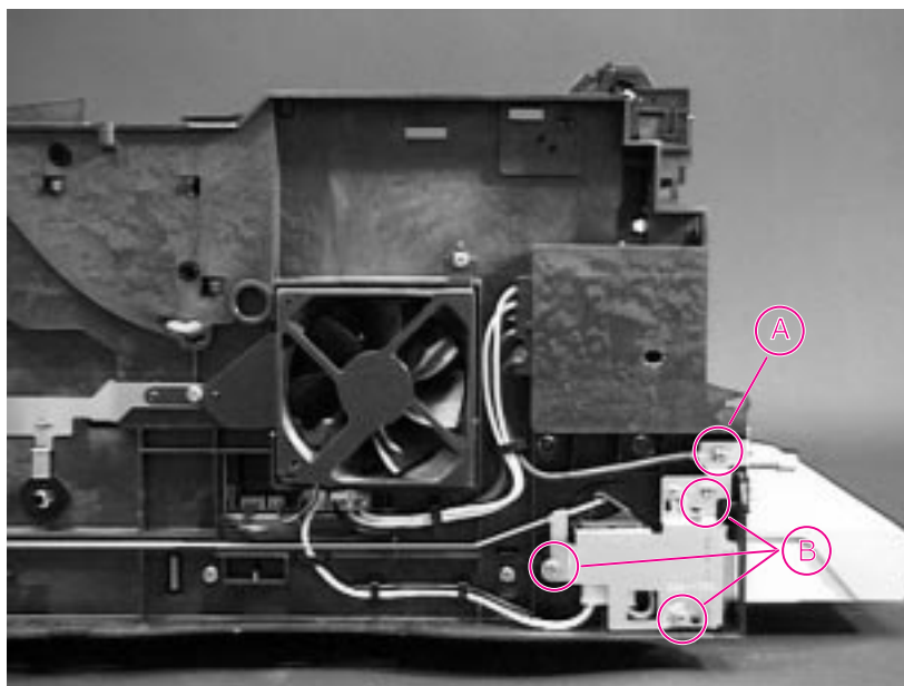
Figure 6-62 Power Inlet Assembly (right side view of printer)
