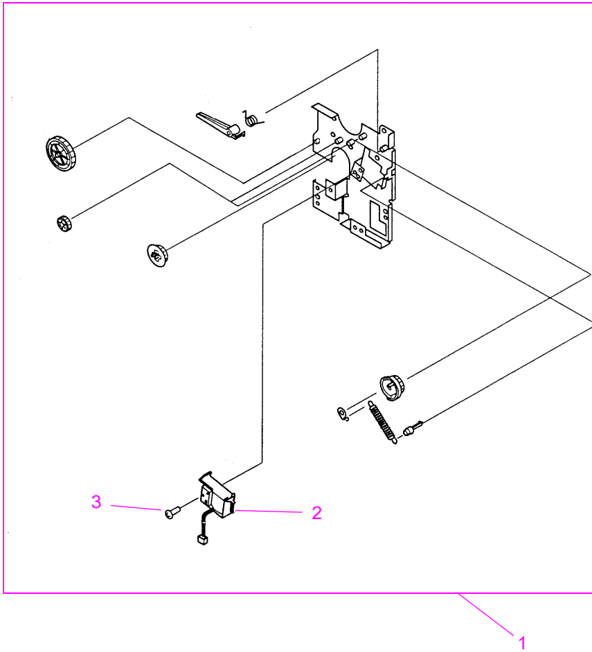
Figure 8-15 Pickup Drive Assembly
