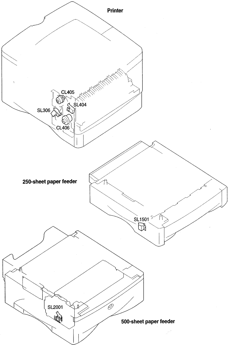
Figure 7-27 Clutches and Solenoids
