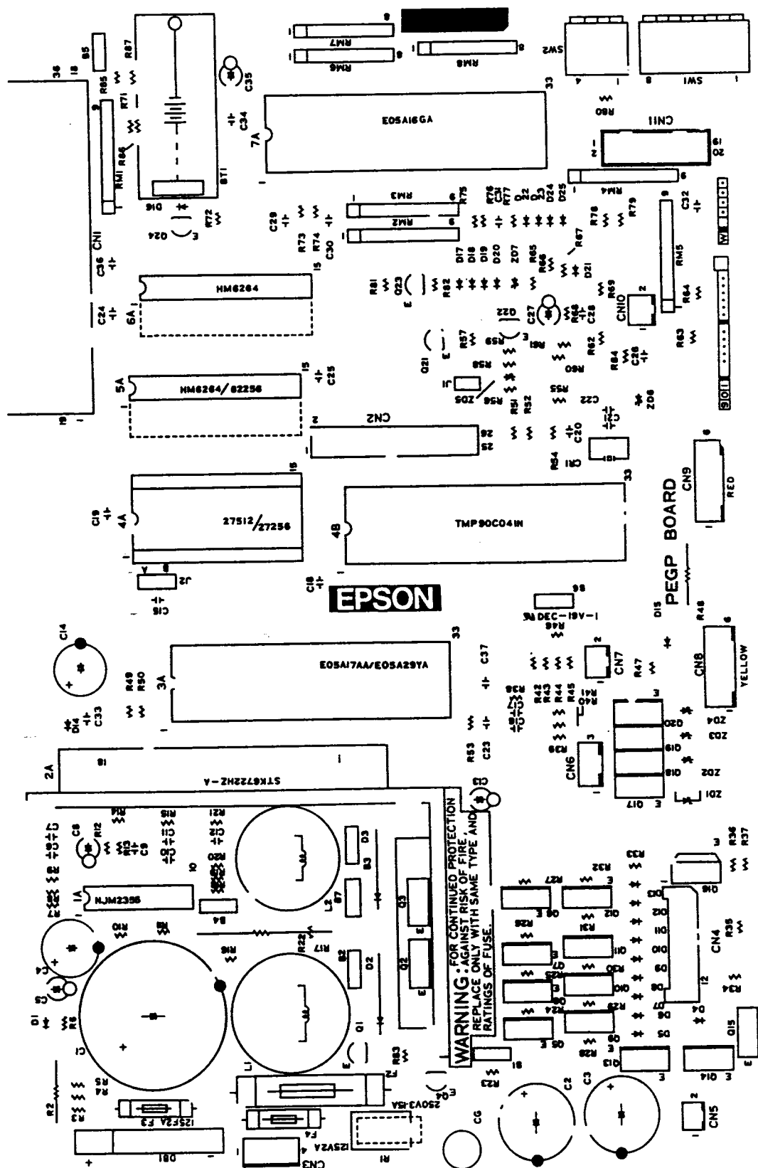
FX850 PEGP BOARD FIG.4
