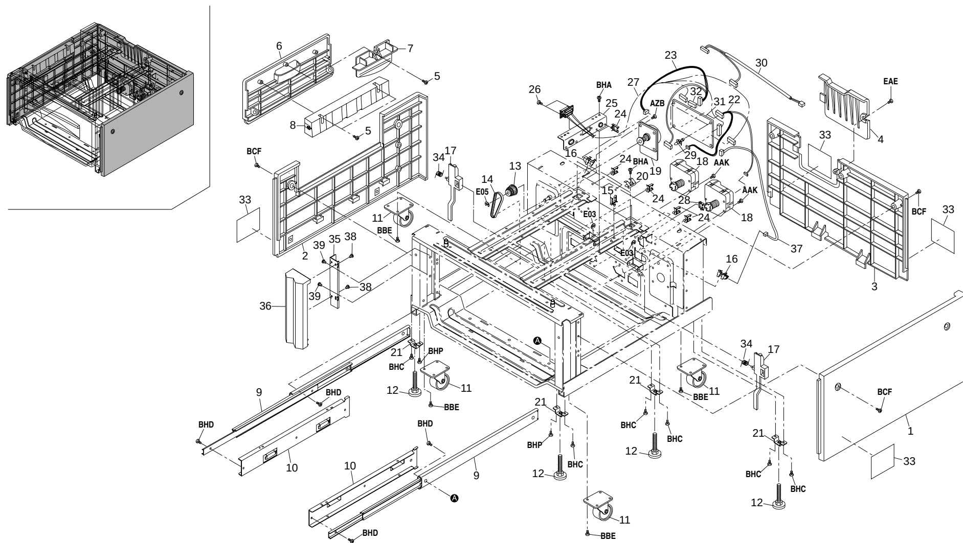
FIG. 1 EXTERIOR COVERS
