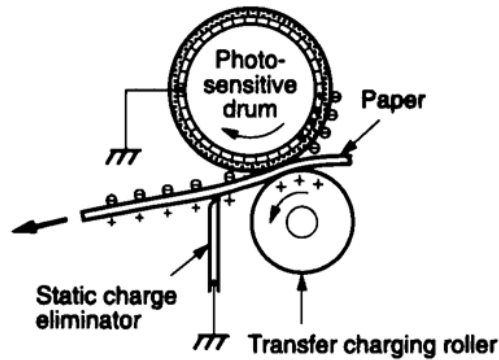
Figure 5-13 Transferring the Toner Image on the Drum Surface to the Paper
