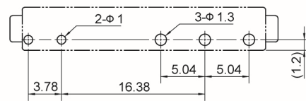
PCB layout (BOTTOM VIEW)
