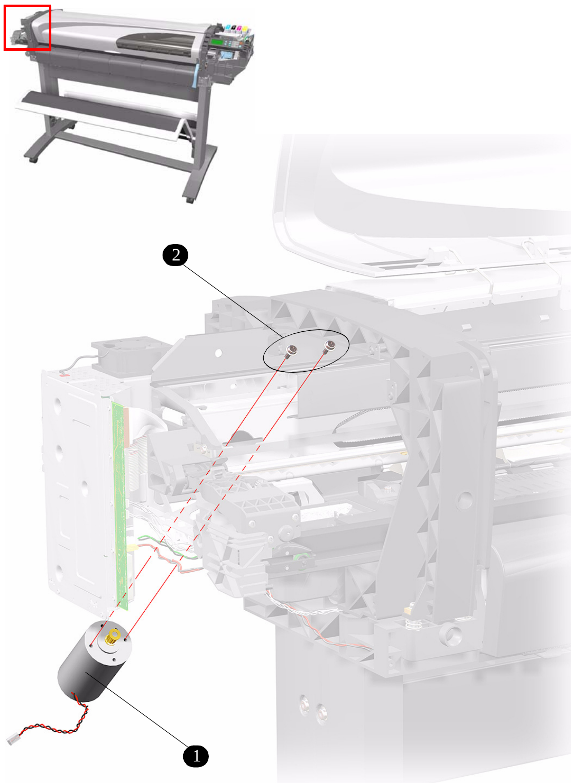
Figure 14: Scan-Axis Motor
