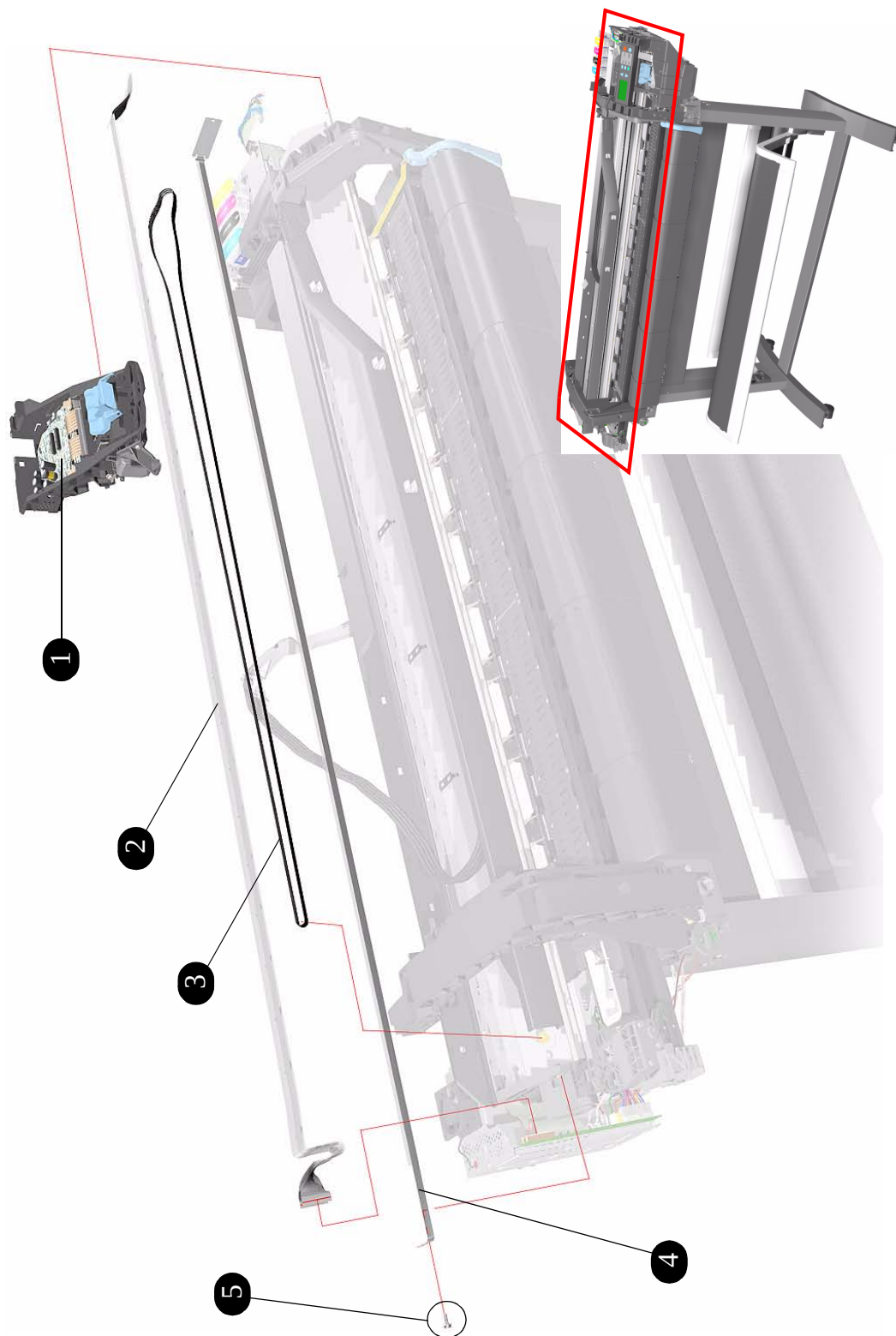
Figure 17: Carriage Assembly
