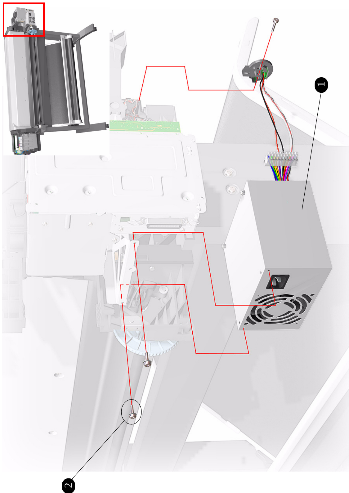
Figure 8: Power Supply
