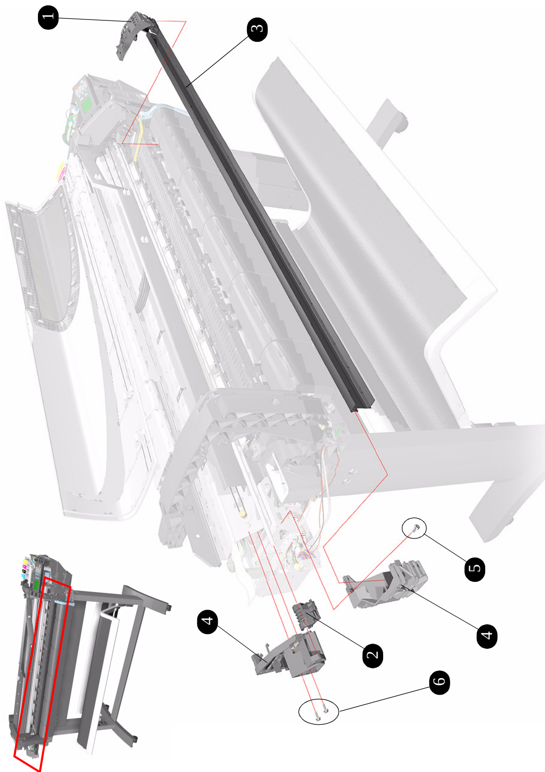
Figure 9: Cutter Assemblies
