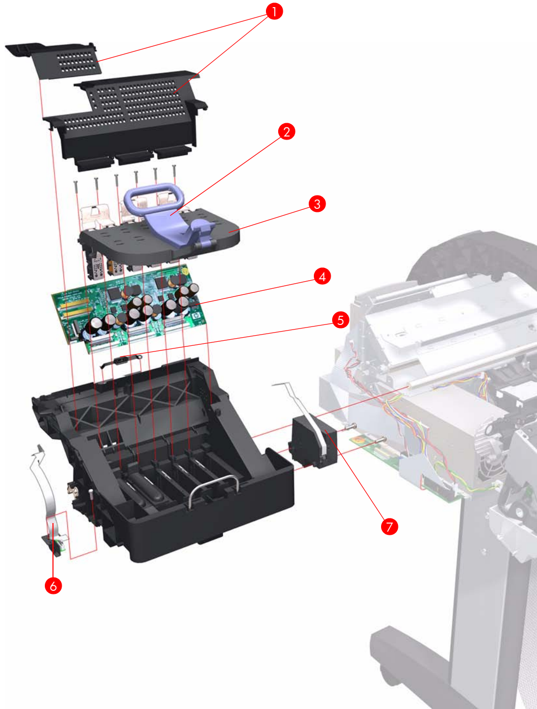
Figure 7-8: Carriage Assembly
