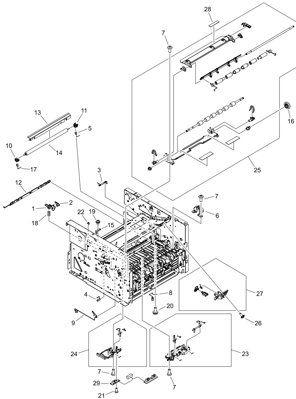
Figure 8-7 Internal components (3 of 4)
