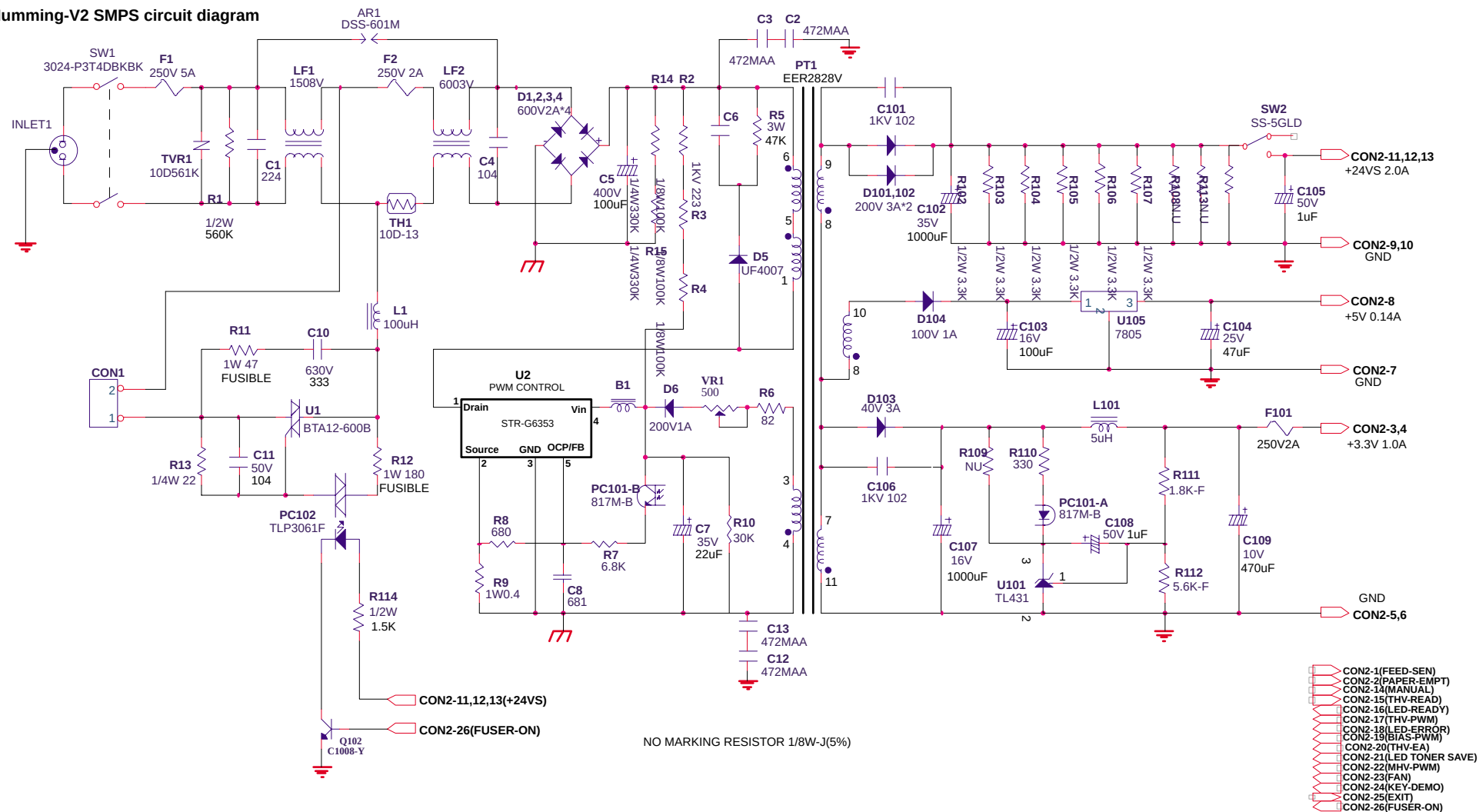
Humming-V2 SMPS circuit diagram
